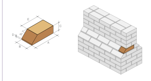
MPL.2 Plinth stretcher faced on end
