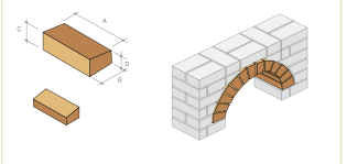
AR.1 Tapered header
