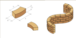
RD.2 Radial stretcher
