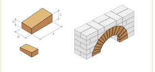
AR.2 Tapered stretcher
