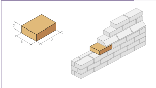
MPL.8 Wide bed stretcher
