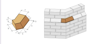
MPL.6 Wide bed plinth external angle
