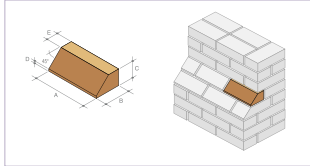
MPL.3 Wide bed plinth stretcher
