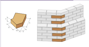
MPL.9 Wide bed external angle
