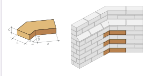
MPL.10 Wide bed internal angle
