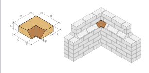
MPL.5 Wide bed plinth internal return
