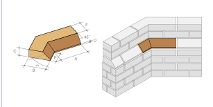
MPL.7 Wide bed plinth internal angle
