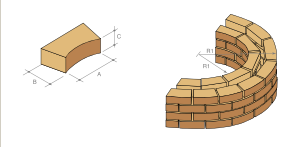
RD.4 Radial stretcher
