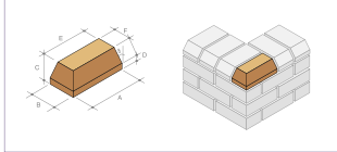
PL.8 Plinth external return
