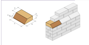
MPL.4 Wide bed plinth external return
